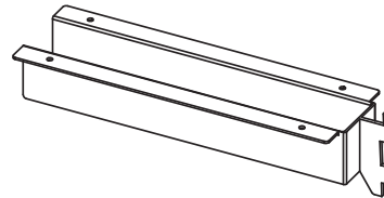
Shelf Bracket Shared RV-SBSHARED13-005
